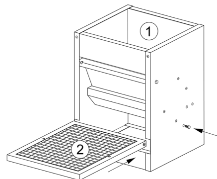
Fig.1 Remove screws of the treadle. Position the treadle, matching the holes of the treadle with the holes of the feeder sides. Insert and tight the screws.
