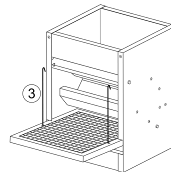
Fig.2 Fix the hooks in place as shown in the figure.
