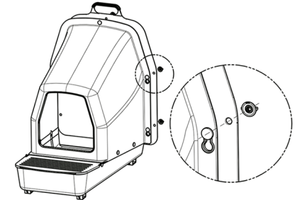
FIGURE 4 Align the black backplate with the holes as shown. Insert plastic viking screw anchor into each hole. Use plastic screws to attach the nesting box to the backplate.
