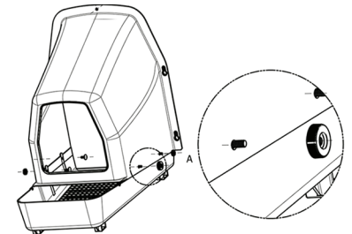
FIGURE 2 Use bolts and plastic nuts to attach nesting box to basket.
